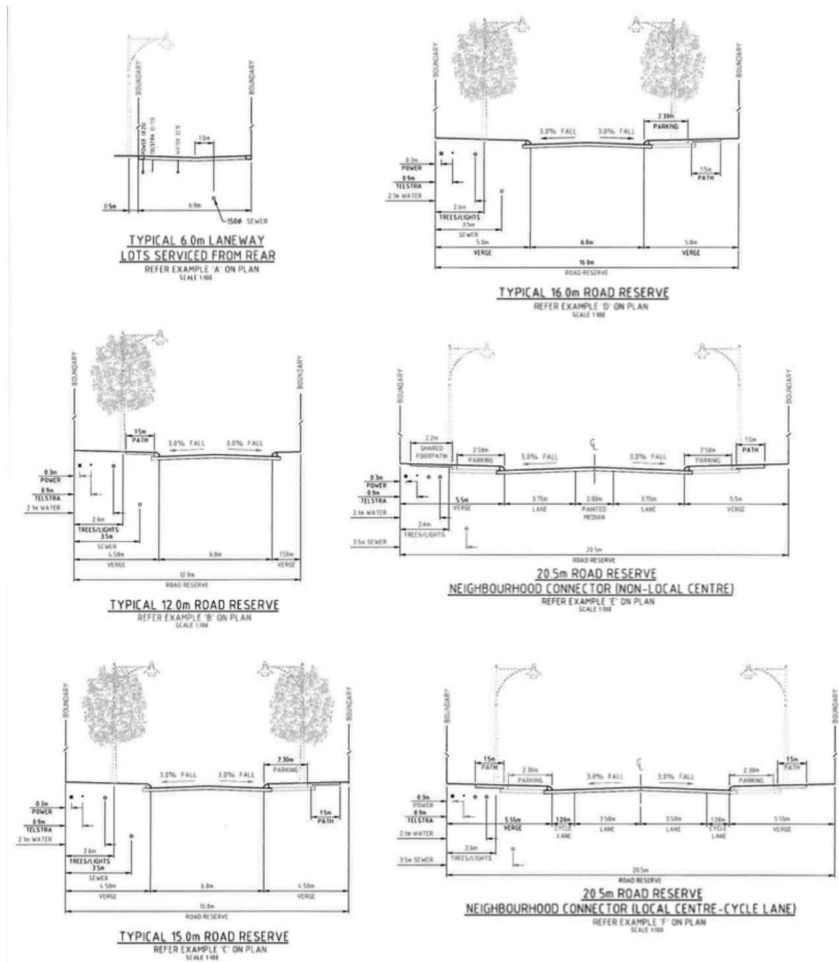
Figure 14 – Indicative street cross sections
